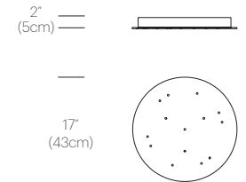
CHANDELIER CANOPY 17"
